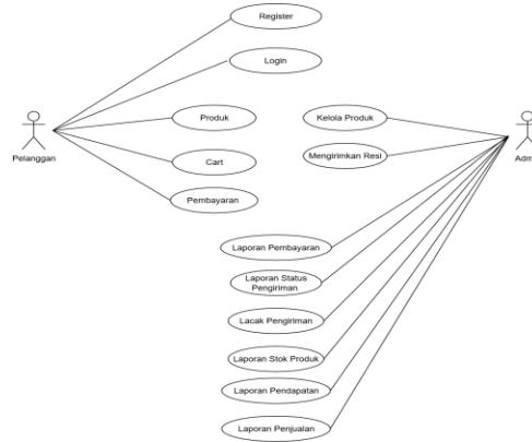
Gambar 2. Usecase diagram website
